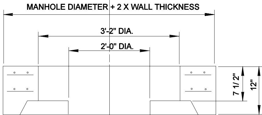
COVER SLAB SECTION
